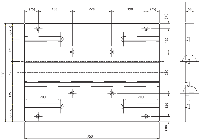
Working table
